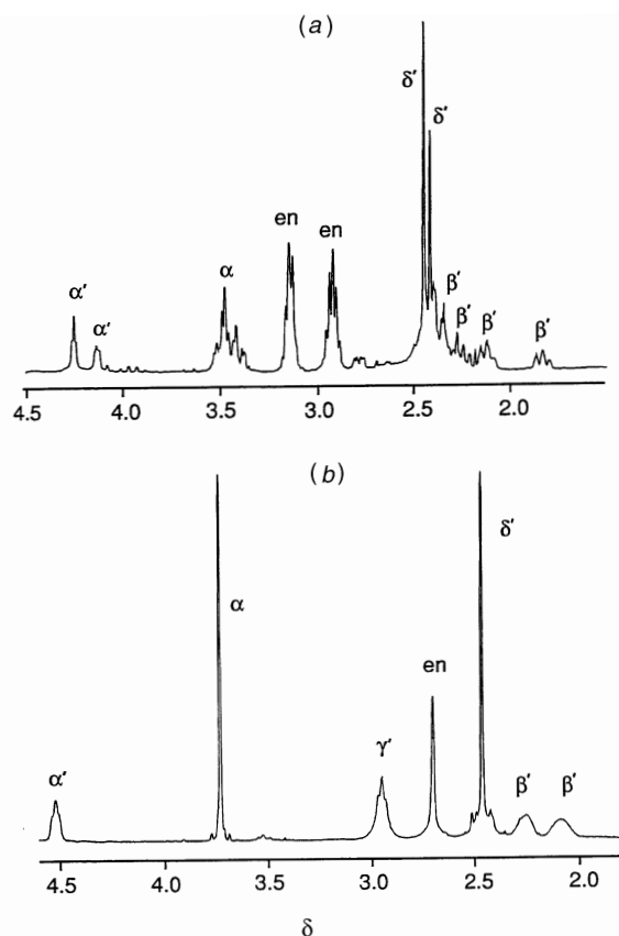
Fig. 7 Proton NMR spectra of (a) [\text{Pt}(\text{Hen-}\kappa\text{N})(\text{gly-met-}\kappa^3\text{N,N',S})]^{2+} and (b) [\text{Pt}(\text{en})(\text{gly-H}_2\text{met-}\kappa\text{S})]^{4+} at pH 2.4
