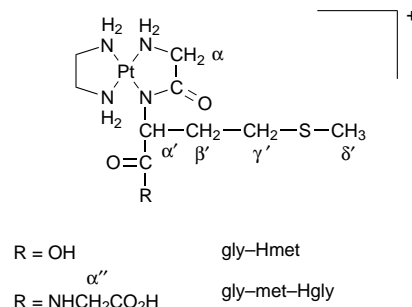
Scheme 6 The \kappa^2\text{N},\text{N}' -co-ordinated complexes for the 1:1 reaction between [\text{Pt}(\text{en})(\text{H}_2\text{O})_2]^{2+} and gly-Hmet or gly-met-Hgly
