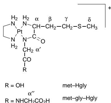
Scheme 2 The \kappa^2N,N' -co-ordinated complexes for the 1:1 reaction systems [Pt(en)(H _2 O) _2 ] ^{2+} -met-Hxaa
