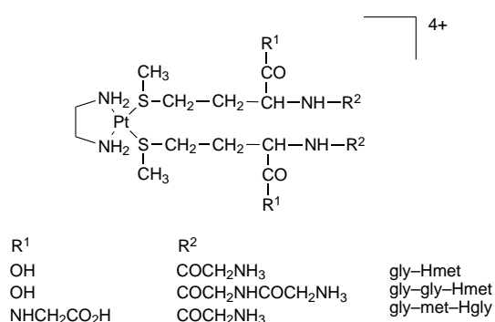
Scheme 5 The (\kappa\text{S})_2 -co-ordinated complexes for the 1:2 reaction systems [\text{Pt}(\text{en})(\text{H}_2\text{O})_2]^{2+} -xaa-Hmet
