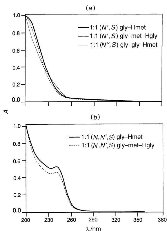
Fig. 6 The UV spectra for (a) \kappa^2 N', S - and \kappa^2 N', S - and (b) \kappa^3 N, N', S -co-ordinated complexes of xaa-Hmet peptides. The absorbances A were normalised
