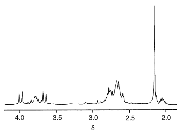
Fig. 4 Proton NMR spectrum of the 1:1 reaction mixture [Pt(en)-(D _2 O) _2 ] ^{2+} -met-Hgly at pH 9.5 [reference sodium (3-trimethylsilyl)tetra-deuteriopropionate, \delta 0.0]
